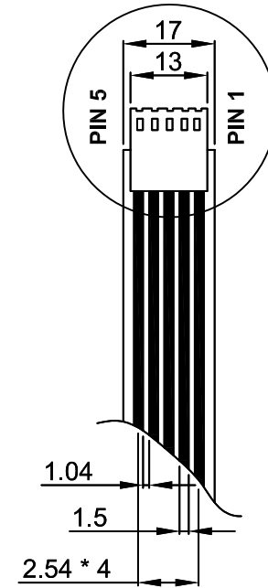
DETAIL A
